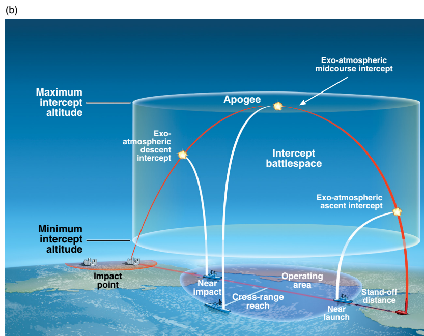
Figure 1. Navy Area TBMD (a) and NTW TBMD (b) battlespace domains illustrating some of the key performance parameters.
